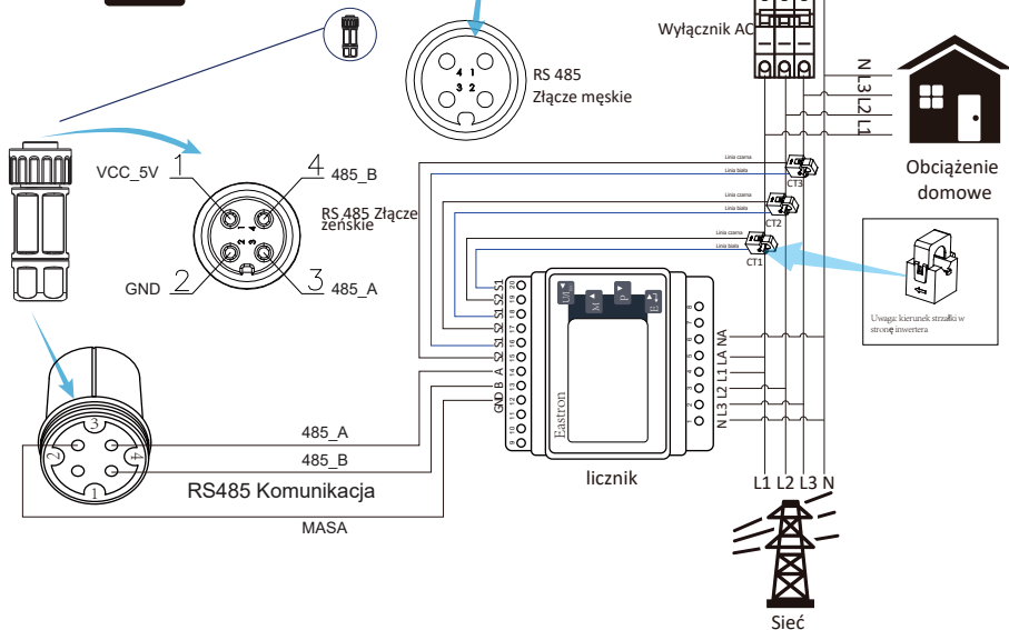
Pic 7.14 Connection diagram of Eastron meter
