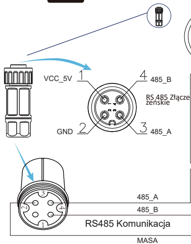
Pic 7.4 Connection diagram of Eastron meter
